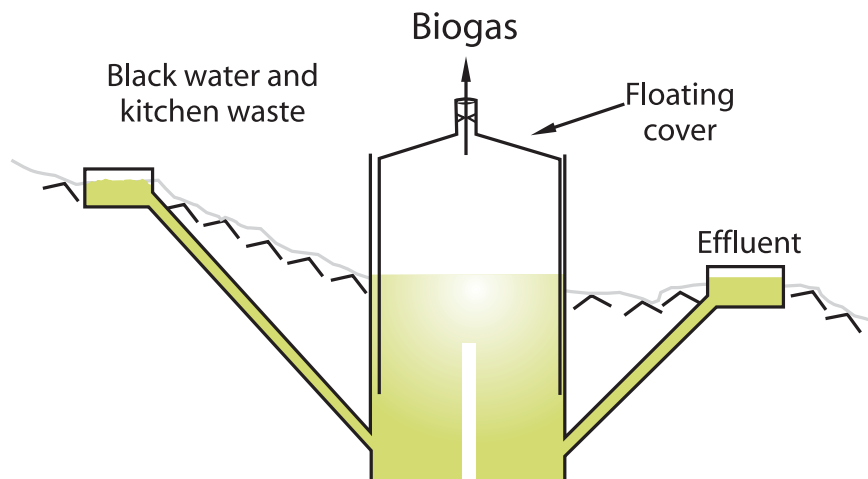
Fig A1.11: Simple system for anaerobic treatment of wastewater
