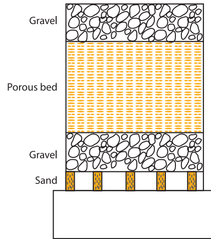
Fig A1.6: Sand filter
