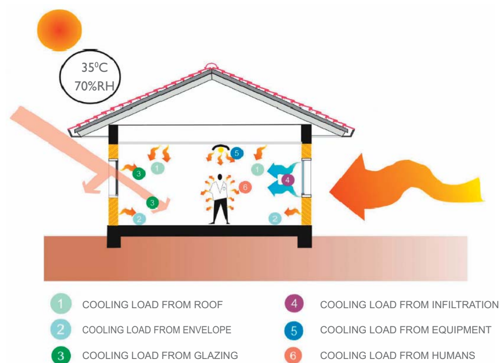
Fig 3.4: Cooling load (Boonyatikarn, S. & Buranakarn, V., 2006)
