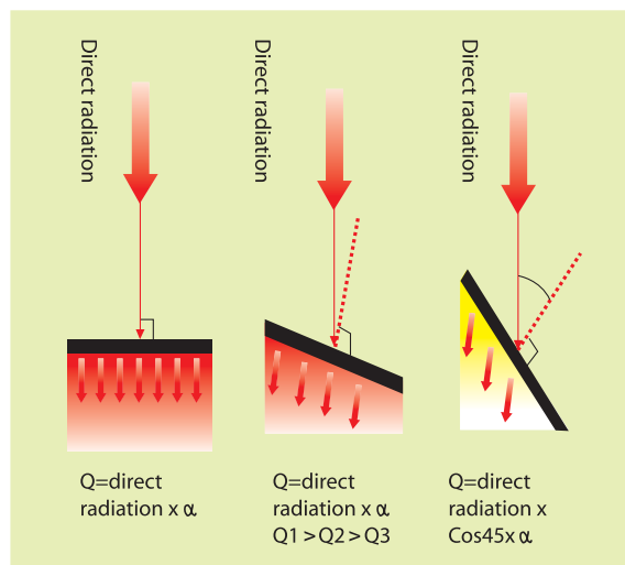
Fig 3.6 a: The impact of roof angle (Boonyatikarn, S. & Buranakarn, V., 2006).
