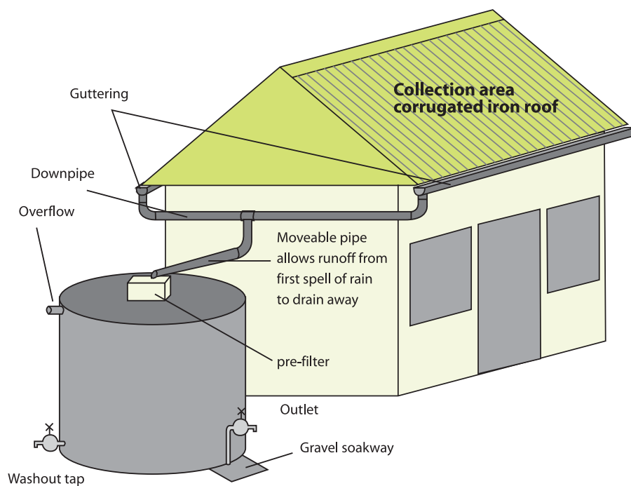
Fig A I.4: Rainwater harvesting system
