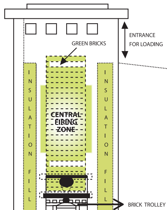
Fig A1.1: Vertical Shaft Brick Kiln
