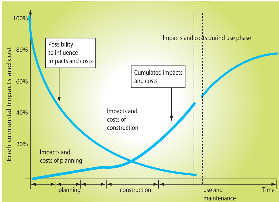
Fig 2.2: Influence of design decisions on life-cycle impacts and costs of an average European and North American building (Kohler,N. & Moffatt, S., 2003, p.14).
