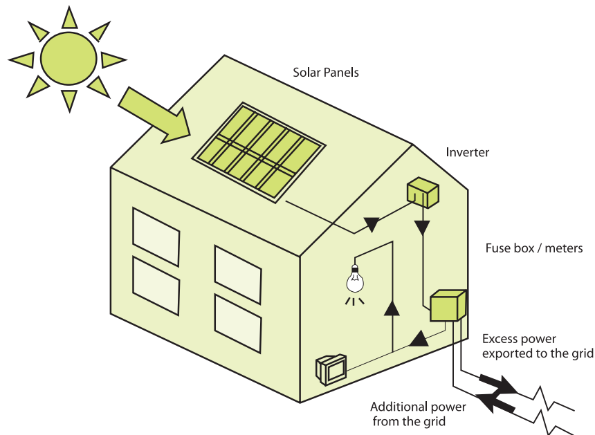
Fig A1.2: A grid connected solar PV system
