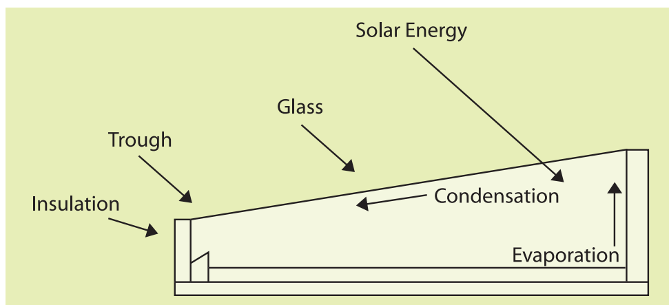
Fig A I.3: Solar still
