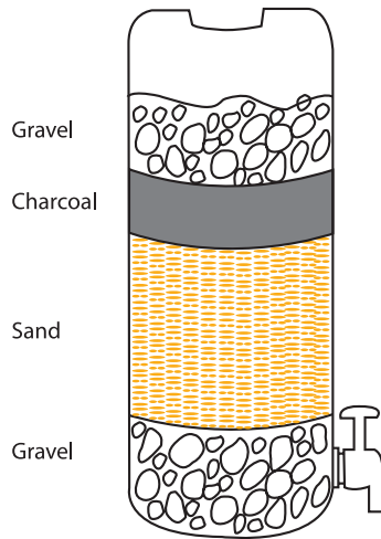
Fig A1.5: Charcoal water filter
