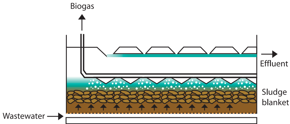
Fig A1.13: UASB reactor
