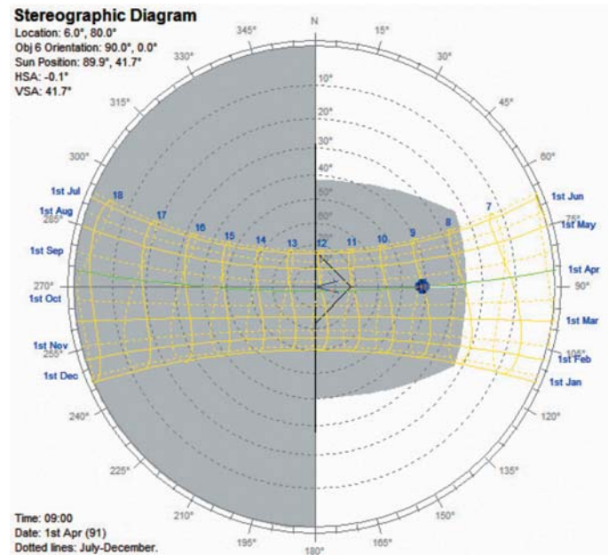
Fig 4.6: Stereographic projection showing shading mask projected by 4'10" shading devices on aperture W1, east façade of the house
