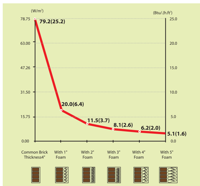
Fig 3.9: Heat Flow through Insulation (Boonyatikarn, S. & Buranakarn, V., 2006)
