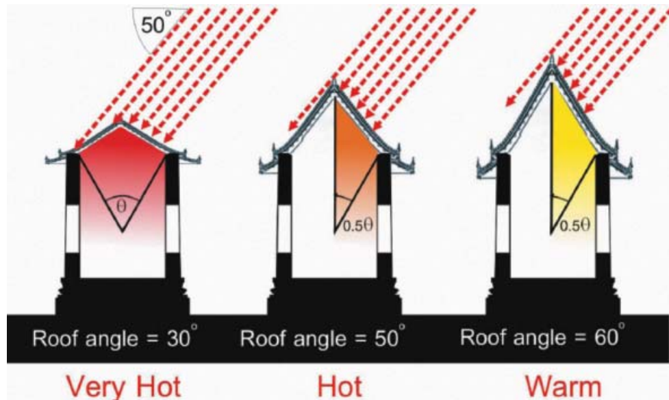
Fig 3.6 b: The impact of roof angle (Boonyatikarn, S. & Buranakarn, V., 2006)
