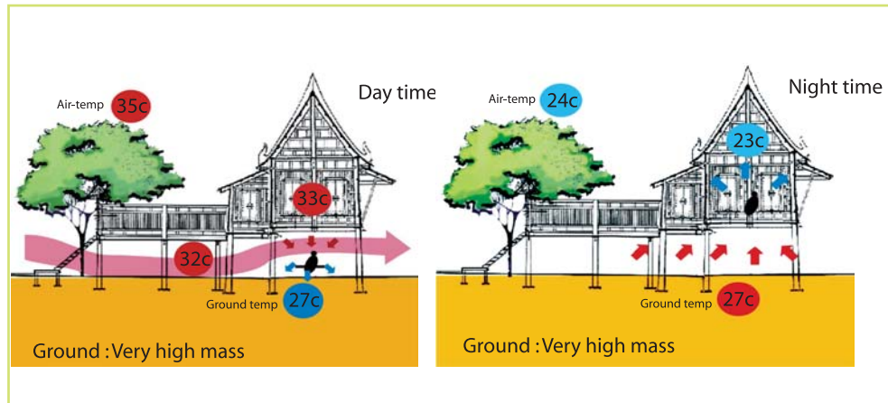
Fig 3.1 I: House on stilts (Boonyatikarn, S. & Buranakarn, V., 2006)
