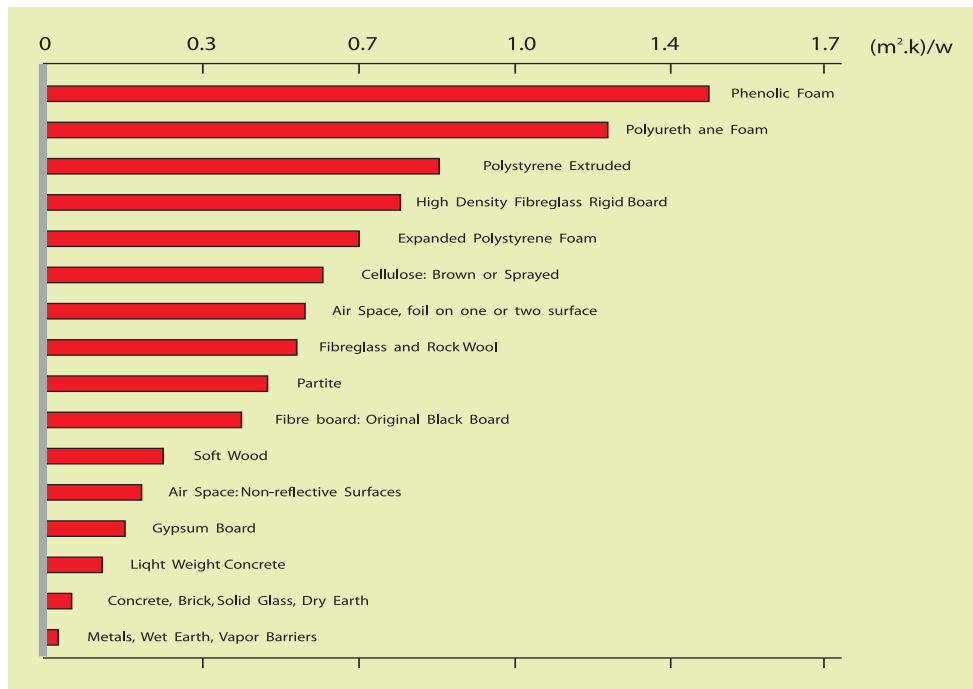
Fig 3.8: Thermal Resistance value (R) for Insulation materials (Boonyatikarn, S. & Buranakarn, V., 2006)
