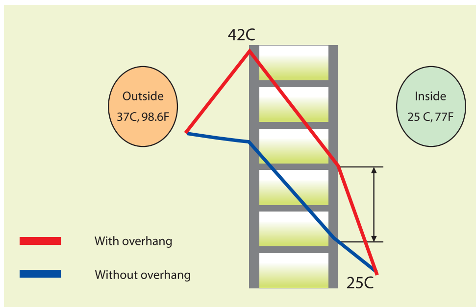
Fig 3.13: Difference in cooling loads, with and without fixed overhangs (Boonyatikarn, S. & Buranakarn, V., 2006)
